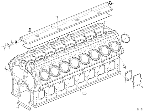
CRANKCASE UPC.06A01 2081
